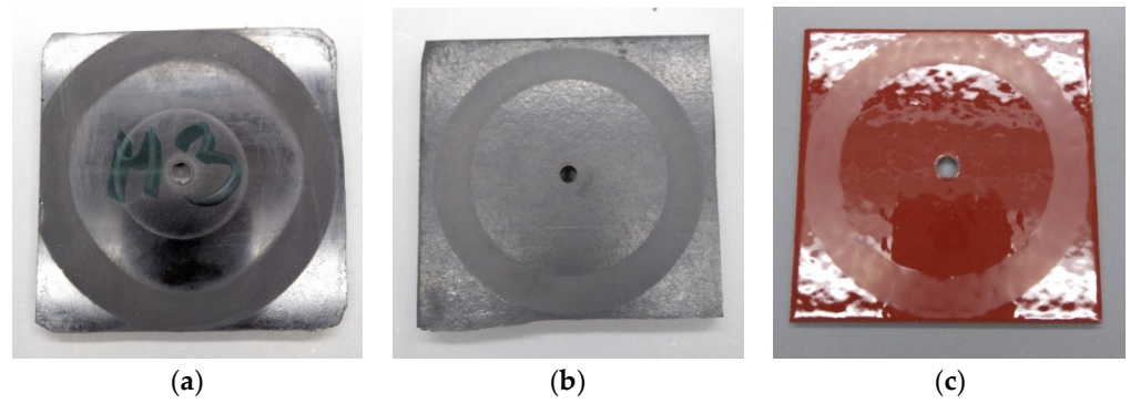
Figure 10. Samples (a): J, (b): K and (c): L after testing.
