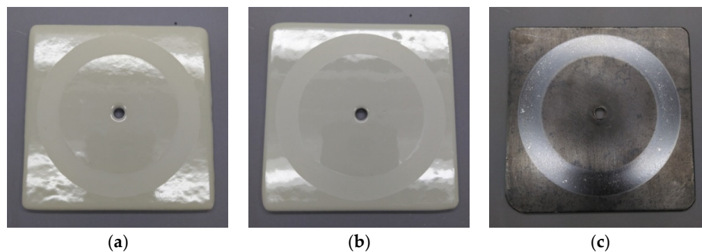
Figure 12. Samples (a): P, (b): R and (c): S after testing.
