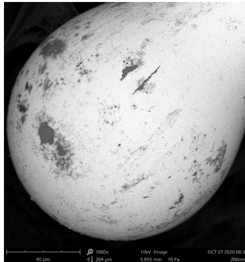
Figure 1. SEM image of the microsphere-sensor with a 100-nm ZnO Atomic Layer Deposition (ALD) coating. Magnification of 1000 \times .
