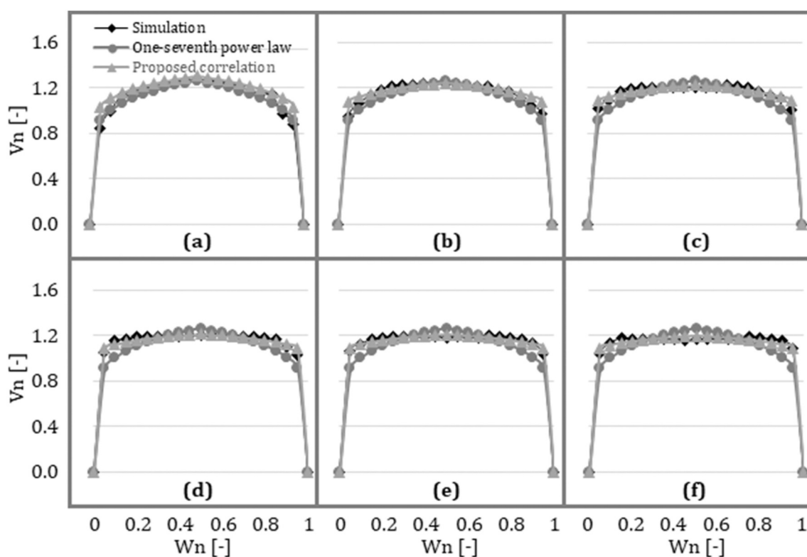
Fig. 13. The normalized velocity profile in I-type flow configuration over the normalized width for constant depth ( d = 0.5 mm) and various aspect ratio (a) \alpha = 2 , D_h = 0.67 mm, (b) \alpha = 5 , D_h = 0.83 mm, (c) \alpha = 7 , D_h = 0.88 mm, (d) \alpha = 9 , D_h = 0.90 mm, (e) \alpha = 10 , D_h = 0.91 mm, (f) \alpha = 12 , D_h = 0.94 mm.
