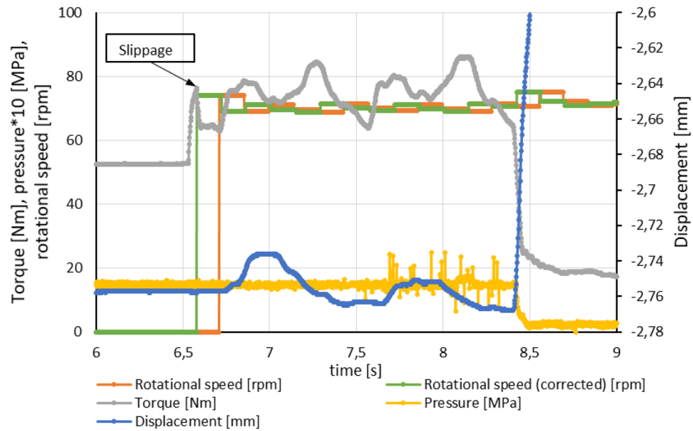
Figure 16. Recorded data of rotational speed, torque, pressure in actuator chamber and displacement presenting decreased displacement of discs package after clutch slippage.
