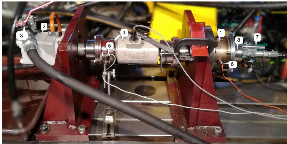
Figure 8. Test stand: 1—multiscap wet clutch testing device, 2—hydraulic motor, 3—shut-off valve, 4—torque transducer, 5—inductive sensor, 6—temperature sensor PT100, 7—displacement sensor, 8—hydraulic actuator.
