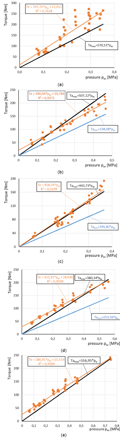
Figure 12. Comparison of torque transmitted by a clutch package formed by discs with different thicknesses as a function of mean value of contact pressure: D_1 = 80 mm, D_o = 115 mm. Number of friction surfaces: (a) 18; (b) 16; (c) 14; (d) 12; (e) 10.
