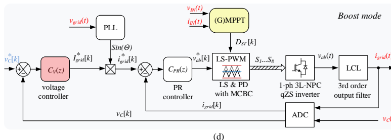
Fig. 2. Examples of the power-voltage curves of the different PV string arrays (a and b) along with proposed control system for buck (c) and boost mode (d) [13].
