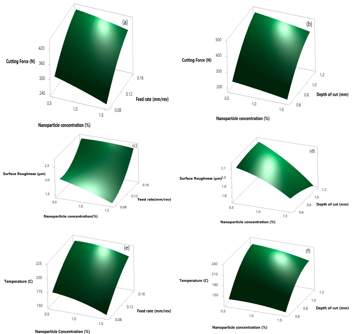
Figure 3. Response surface plot for alumina nanofluid for cutting force. (a) np% Vs f_o ; (b) np% Vs a_p ; for surface roughness (c) np% Vs f_o ; (d) np% Vs a_p and for cutting temperature (e) np% Vs f_o ; (f) np% Vs a_p .
