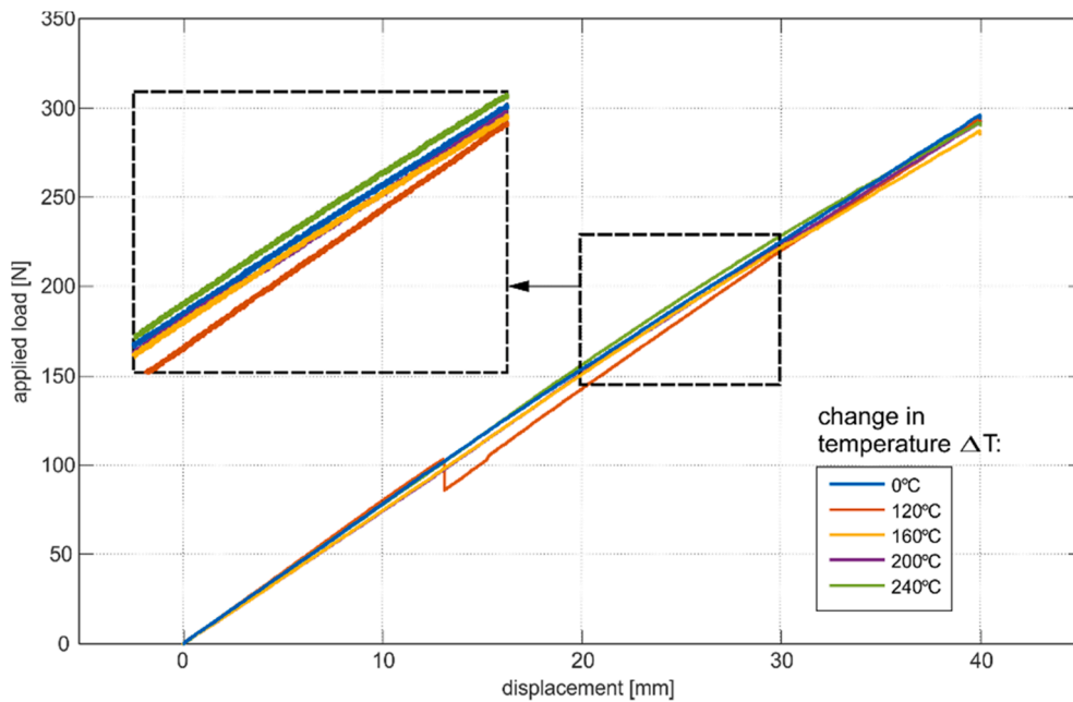
Fig. 6. Results of bending tests of cooled GFRP bars: load–displacement curves.
