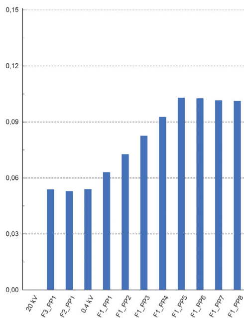
Total Harmonic Distortion in %
