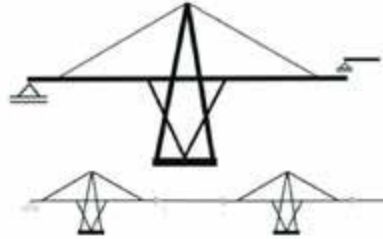
Fig. 27. Viaduct in Genoa, Italy, 1967 (photo: Google Maps, July 1998) and a schema of bridges developed by R. Morandi
