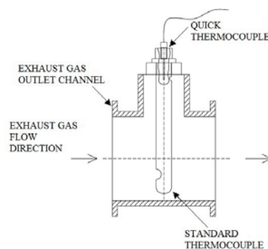
Fig. 2: (a) General view of exhaust gas ducts supplying a marine diesel engine turbocharger in a pulse system with a place for mounting standard thermocouples and (b) schematic diagram of adaptation of a standard thermocouple by mounting a thermocouple for high-speed measurements
