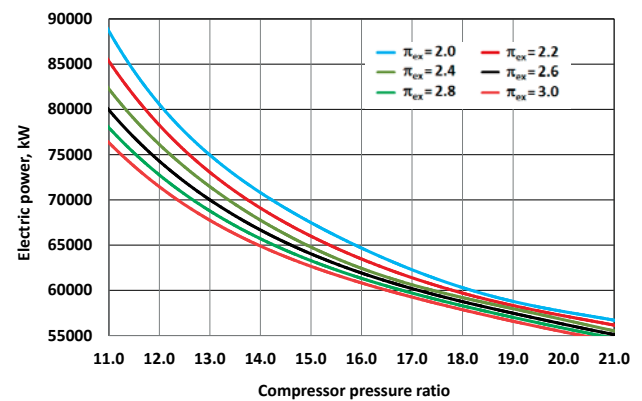
Fig. 3. Dependences of the electric power of the combined CGSTU of a hybrid cycle on the compressor and exhauster pressure ratios.
