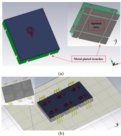
FIGURE 22. (a) 2 x 3 loop-antenna array layout, and (b) silicon area and metal plated trenches [92].
