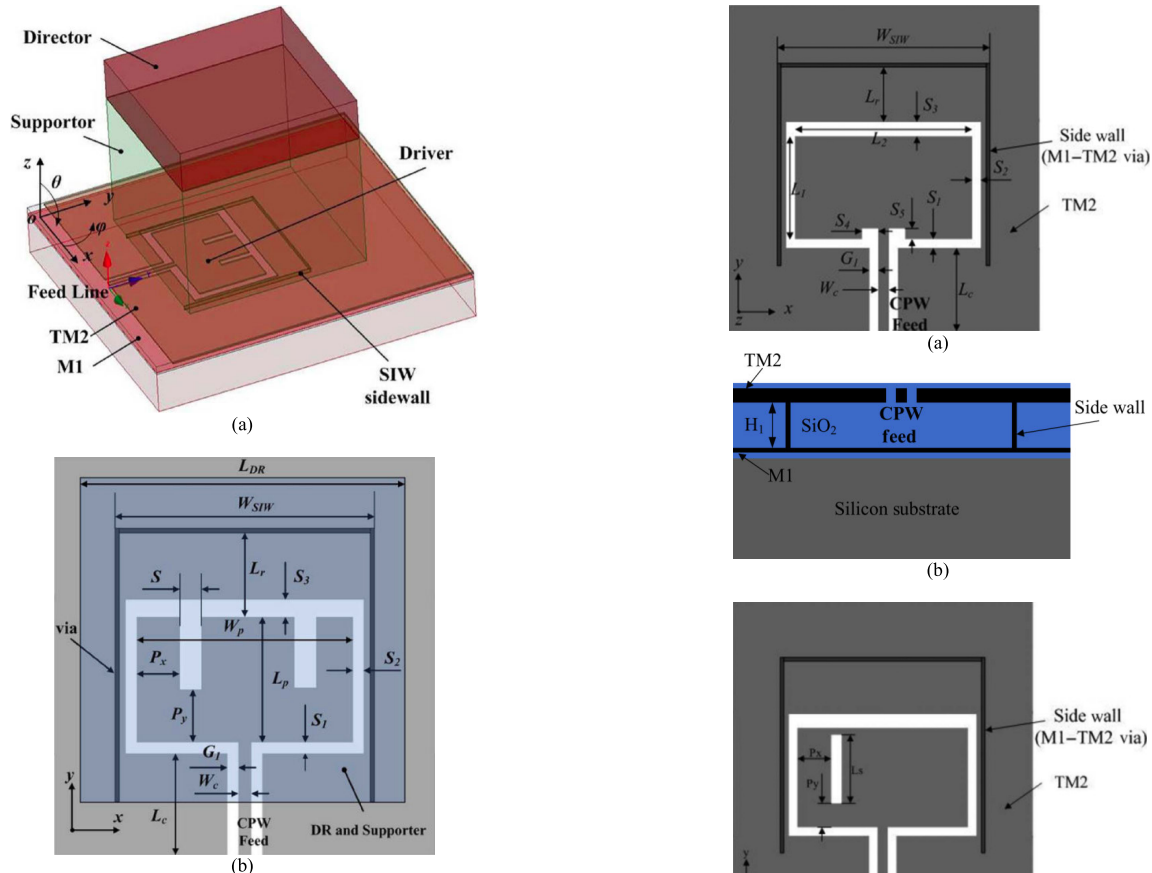
FIGURE 2. Configuration of the 3-D antenna on-chip constructed of an on-chip driver and a dielectric resonator director: (a) three dimensional view, and (b) top side [89].
