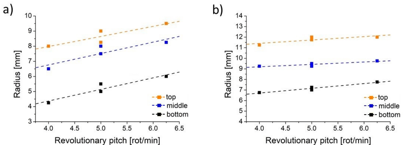
Figure 8. Radius of the nugget zone as a function of revolutionary pitch—relationship for the friction stir welds produced with the tilt angle 0^\circ (a) and 2^\circ (b).
