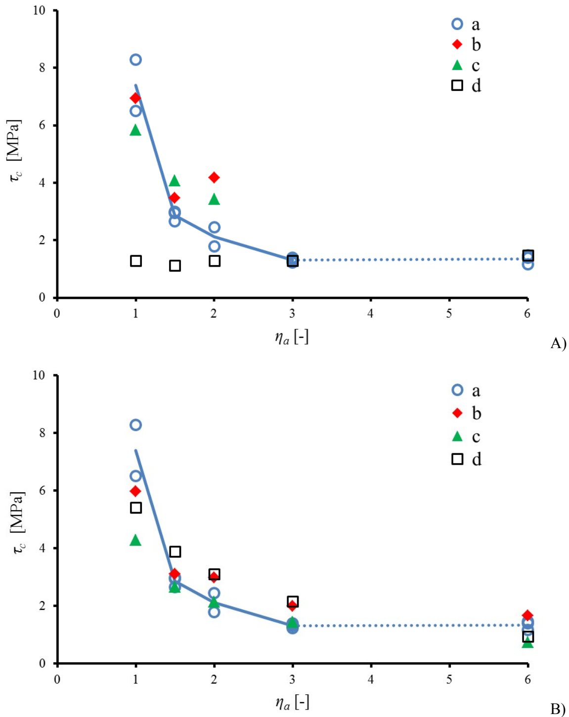
Fig.A1.18: Shear strength \tau_c = V_{max}/(tD) ( V_{max} = 0.5P_{max} ) for varying shear span parameter \eta_a = a/D in experiments (a) and in analytical solutions: A) codes ((b) ACI (Eqs.A1.7-A1.9), c) STM (c) (Eqs.A1.10 and A1.11) and d) EC2 (Eqs.A1.5 and A1.6)) and B) alternative formulae (b) alternative ACI (Eq.A1.14), c) alternative STM (Eq.A1.16) and alternative STM (Eq.A1.17) (note that beams for \eta_a = 6 failed in flexural mechanism)
