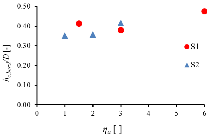
Fig.A1.10: Experimental normalized mean height of compressive zone h_c/h in RC beams for series '1' (S1; marked with dots) and '2' (S2, marked with triangles) in shear zone (a) and bending zone (b) versus \eta_a = a/D ( a - shear span, D - effective height)
