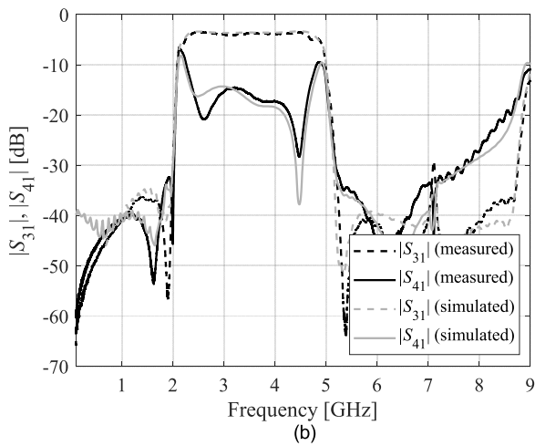
FIGURE 7. EM-simulated and measured performance of the proposed FBLC: (a) |S_{11}| and |S_{21}| , (b) |S_{31}| and |S_{41}| .
