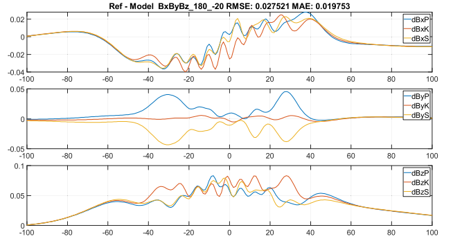
FIGURE 37. Ref-model differences on paths in nT: S7, direction 180^\circ .
