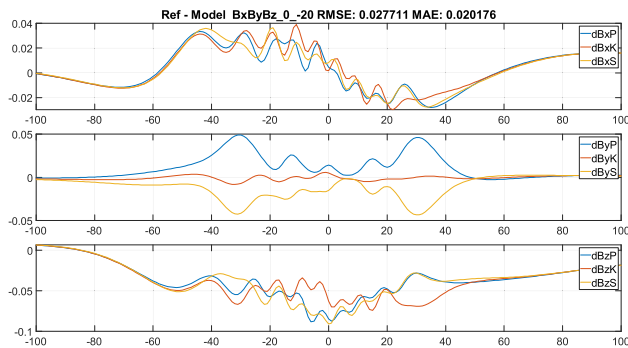
FIGURE 33. Ref-model differences on paths in nT: S7, direction 0^\circ .
