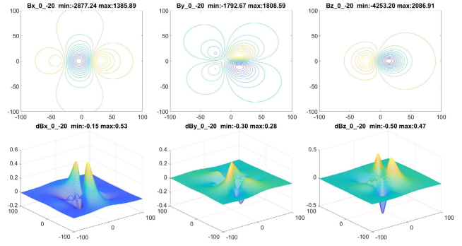
FIGURE 34. Ref-model differences on fields in nT: S7, direction 0^\circ .
