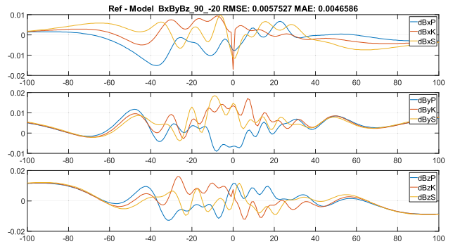
FIGURE 35. Ref-model differences on paths in nT: S7, direction 90^\circ .
