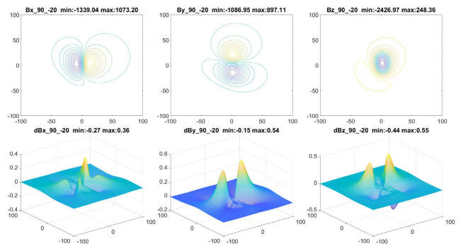
FIGURE 36. Ref-model differences on fields in nT: S7, direction 90^\circ .
