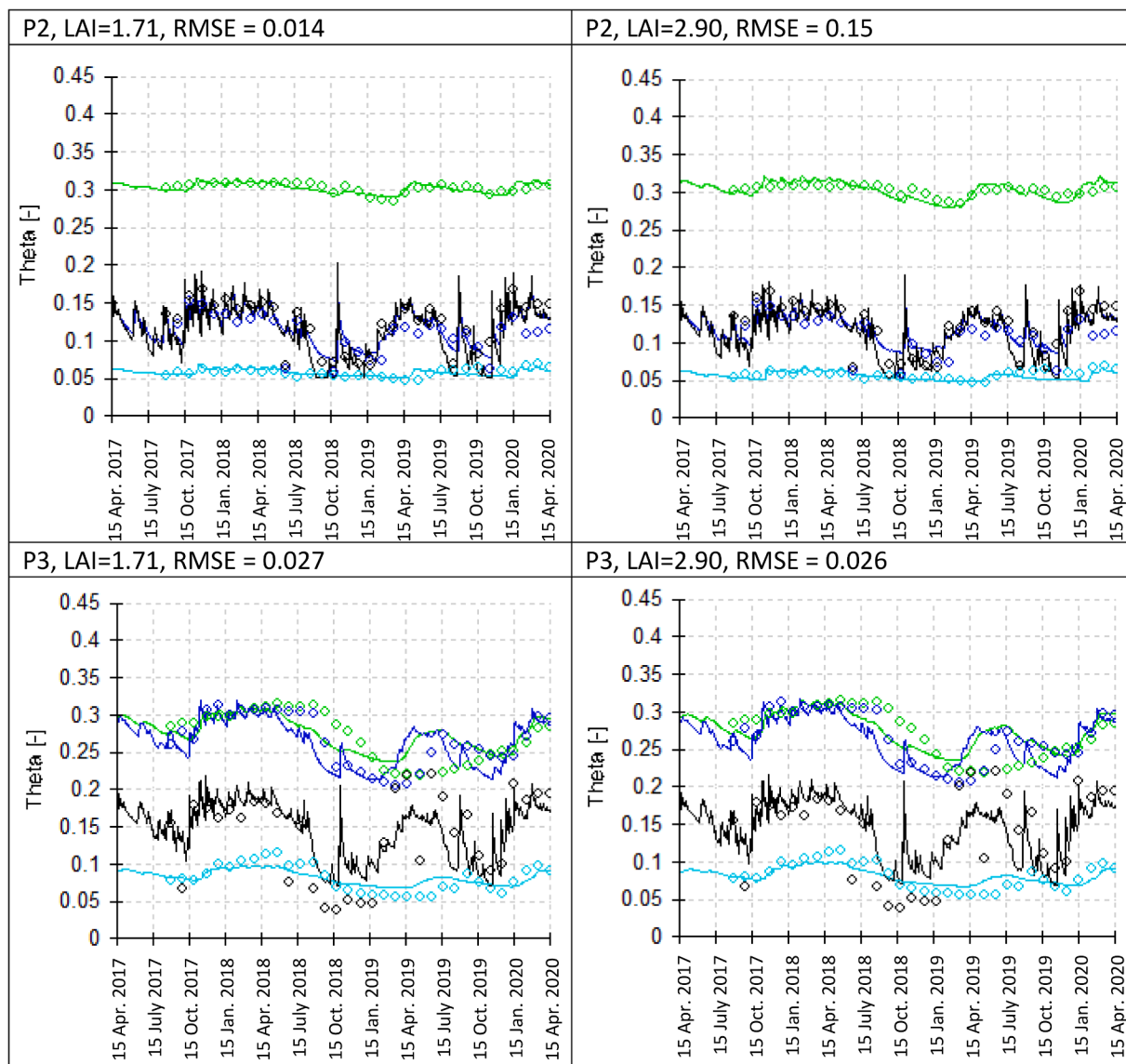
Fig. 4. Measured and simulated water contents in the grassland profiles P2 and P3 (sensor depth: 2P –20 cm (black), 50 cm (dark blue), 150 cm (green), 450 cm (light blue), and 3P – 10 cm (black), 90 cm (dark blue), 180 cm (green), 280 cm (light blue)).
