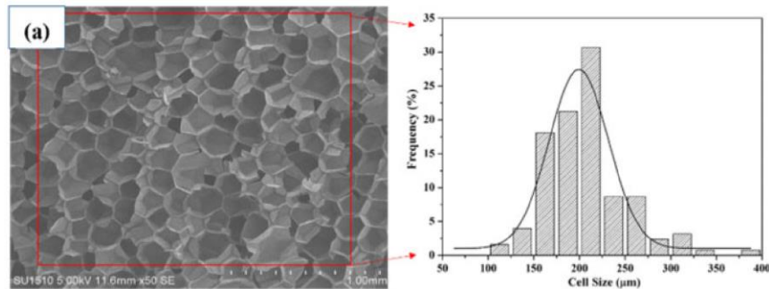
Fig. 6. SEM microphotograph of the pure PF surface and cell distribution [11].
