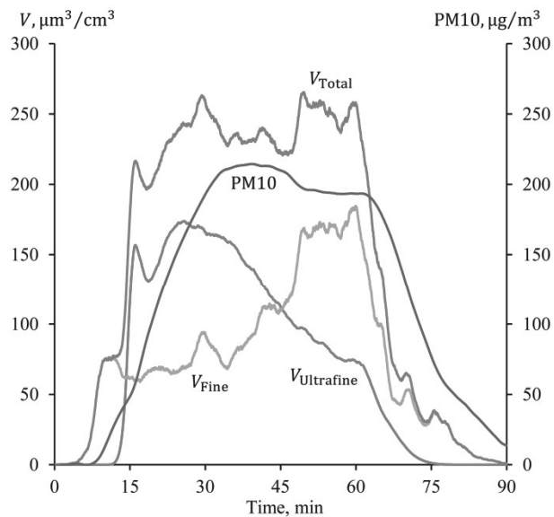
Fig.5. Particle volume concentrations V_{\text{Fine}} and V_{\text{Ultrafine}} and PM10 vs. time (M1, 1.5 MPa × 1.6 m/s) (colour online only)
