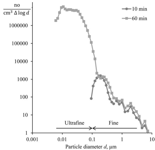
Fig.4. Particle size distributions (M1, 1.5 MPa × 1.6 m/s) (colour online only)
