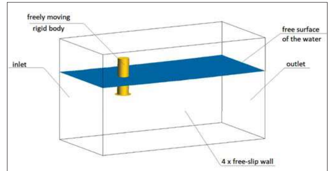
Fig. 2. Computational domain
