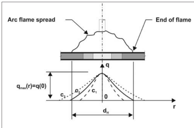
Fig. 11. Model of disc source of heat [26]
