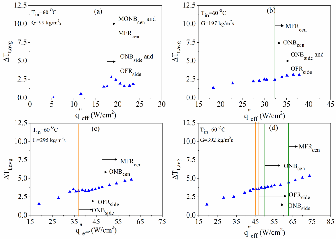
Fig. 21 Effect of heat flux on average transverse temperature difference at different mass fluxes and T_{in} = 60 °C.
