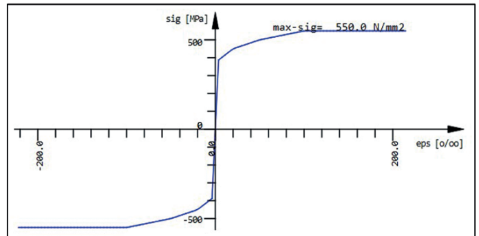
Work law for nonlinear QUAD-elements Mno: 1
