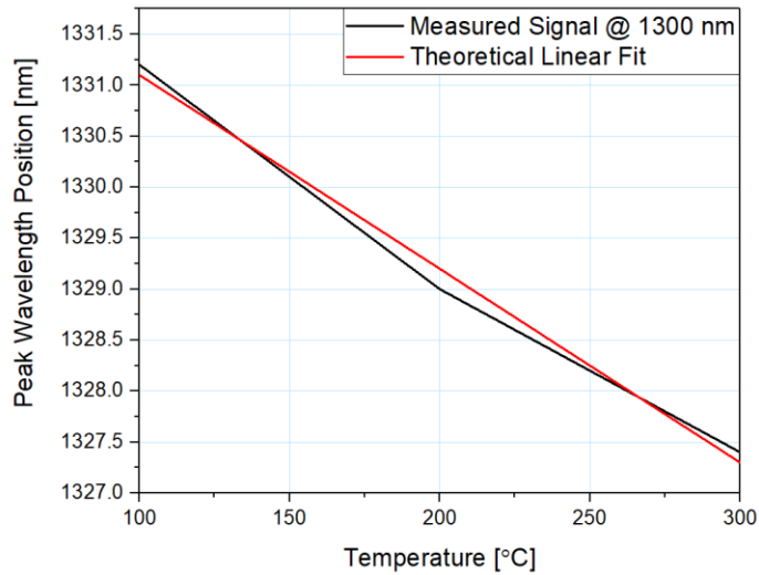
Figure 4.9. Dependence of the spectral shift of a reflected signal on the temperature.
