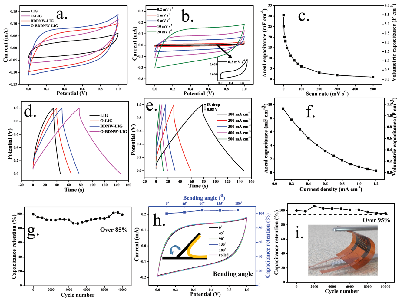
Figure 4. Electrochemical performance of MSCs in PVA- \text{H}_2\text{SO}_4 electrolyte. a) Comparison of the CV profiles of LIG, O-LIG, BDNW-LIG, and O-BDNW-LIG at a scan rate of 10 \text{ mV s}^{-1} . b) CV curves of O-BDNW-LIG at different scan rates. c) Areal and volumetric specific capacitance of O-BDNW-LIG as a function of scan rate. d) Comparison of the GCD curves of LIG, O-LIG, BDNW-LIG, and O-BDNW-LIG at a current density of 0.1 \text{ mA cm}^{-2} . e) GCD curves of O-BDNW-LIG at a current density range of 0.1\text{--}0.5 \text{ mA cm}^{-2} . f) Areal and volumetric specific capacitance of O-BDNW-LIG calculated from GCD curves as a function of current density. g) Cyclic stability of O-BDNW-LIG over 10 000 charge/discharge cycles. h) CV curves of O-BDNW-LIG under different bending conditions at 20 \text{ mV s}^{-1} . Mechanical stress does not affect its electrochemical performance. i) Cyclic stability of O-BDNW-LIG under bending conditions. The bent device retains 96% of its initial capacitance after 10 000 charge/discharge cycles. The inset of (i) shows a snapshot of the O-BDNW-LIG MSC device bent with a tweezer.
