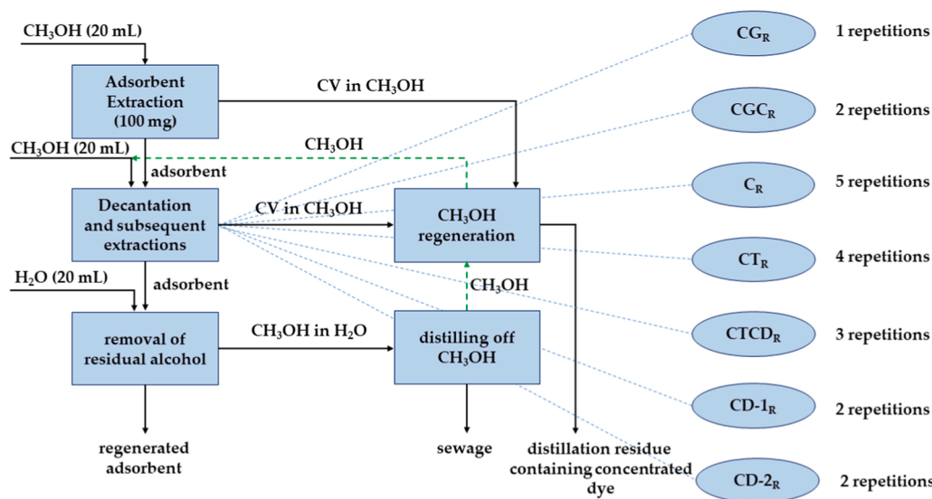
Scheme 2. A simplified schematic diagram of the adsorbent regeneration process.
