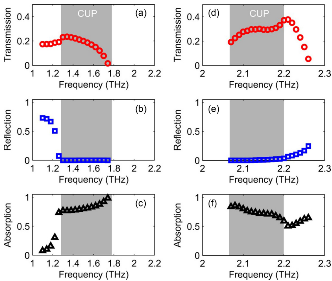
FIG. 4. Transmission, reflection and absorption coefficients, inside and near the complete unidirectional propagation (CUP) band (grey area), for a 2 μm slit of (a)–(c) the unidirectionally guiding (nontopological) structure; and (d)–(f) the unidirectionally guiding topological structure, for the optimum respective slit positions in both cases. Note that in both cases the reflection coefficient inside the CUP band is virtually zero as it should be from theory.
