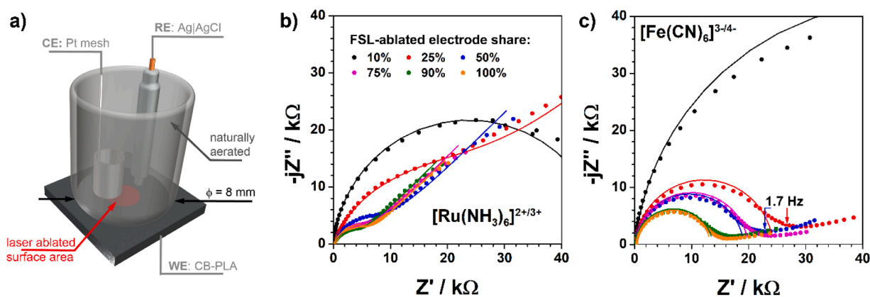
Fig. 4. (a) The scheme of the electrochemical cell used for the measurements, with FSL-ablated area marked in red; (b,c) EIS Nyquist plots of CB-PLA with different FSL-ablated electrode shares between 10 and 100%, studies in the presence of (b) 1 mM [\text{Ru}(\text{NH}_3)_6]^{2+/3+} and (c) 2.5 mM [\text{Fe}(\text{CN})_6]^{3-/4-} . Laser ablation parameters for E100 sample: E_i = 20.1 \mu\text{J} , \nu = 2500 \text{ mm s}^{-1} , 1 scan.
