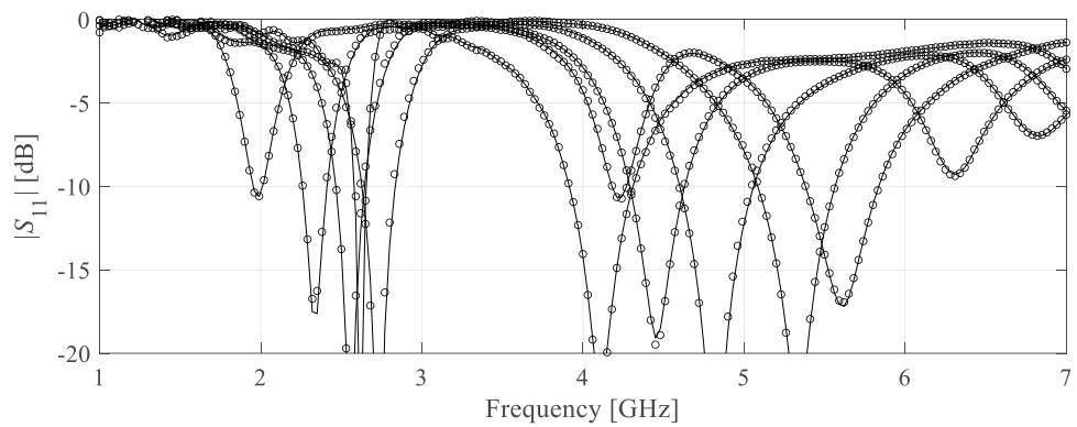
Figure 13. Antenna II: reflection responses at the representative test designs: full-wave model (—), and the presented two-level variable-fidelity surrogate (o) with N_{Bf}=50 and N_{Bc}=800 .
