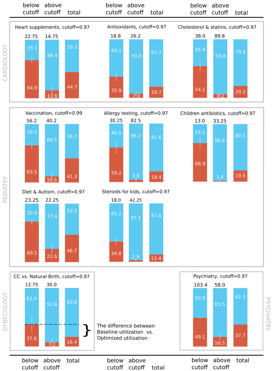
Fig. 3 Cross-validated proportions of positive and negative samples (a) below the cutoff (b) above the cut-off (c) in the entire test set. This corresponds to precision for the negative class, precision for the positive class and total label proportions, respectively. Black labels indicate the mean number of samples in each group. Each bar has the standard deviation indicator (white vertical line)
