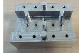
Fig. 5. Photograph of the manufactured prototype (internal dimensions: 22.86 \times 36.58 \times 10.16 \text{ mm}^3 ).
