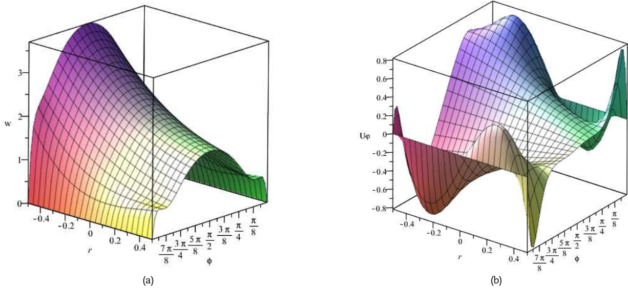
Fig. 6. Movement of the Earth's layers under pressure applied on common boundary between the outer core and lower mantle for (a) radial w (b) shear U_\varphi displacement.
