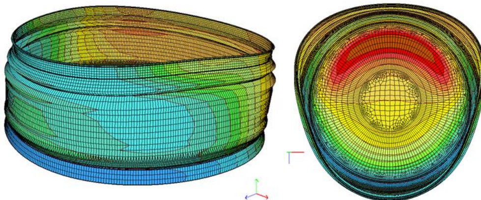
Fig. 6. The map of nodal deflections due to weakening of KZ2 and KZ3 regions, 80% with regard to the averaged subsoil stiffness modulus
