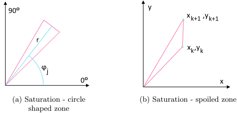
Fig. 2: Inequality constraints - azimuth thruster
