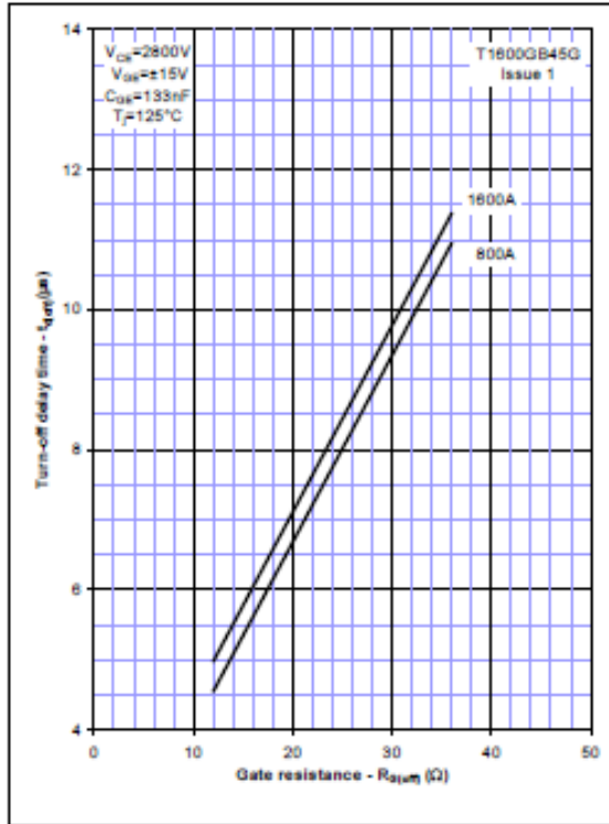
Figure 5 – Typical turn-off delay time vs. gate resistance
