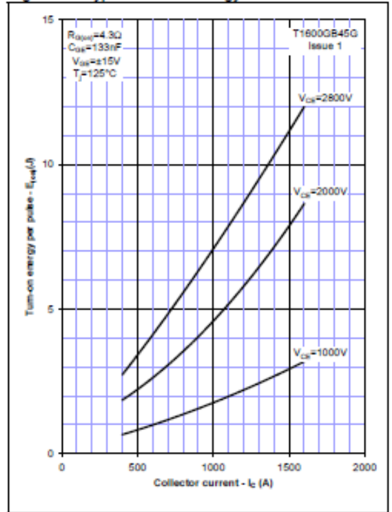
Figure 6 – Typical turn-on energy vs. collector current
