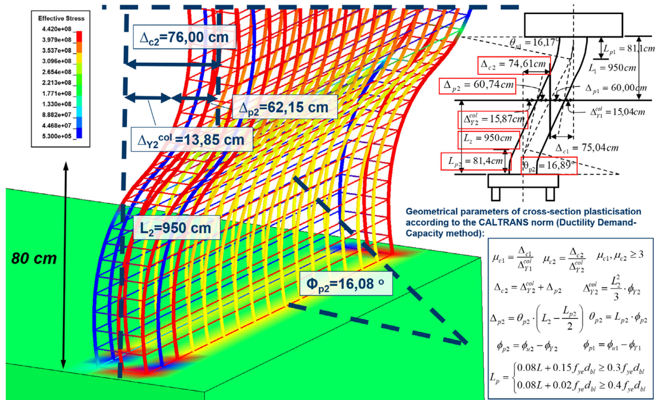
FIGURE 17 Local displacement capacity - lower hinge
