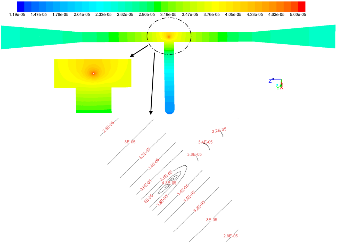
Fig 13. Electric charge contour at voltage 30 KV
