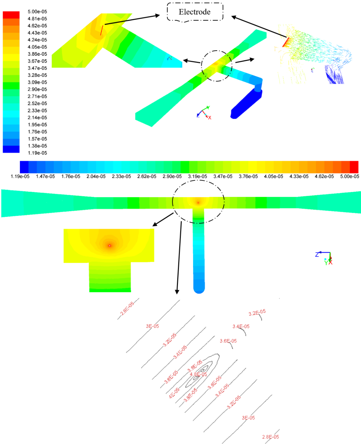
Fig 13. Electric charge contour at voltage 30 KV
