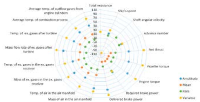
Fig. 13. Relative changes in the statistical parameters of the system variables (in percentages) under propeller ventilation
