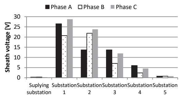
Fig. 6 Sheaths voltages for alternatively cross-bonded sheaths
