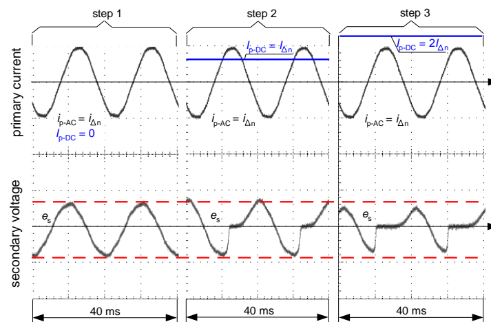
Figure 17. Oscillograms of the induced secondary voltage e_s in case of the iron core of flat hysteresis loop (as in Figure 15b). Primary current i_p composed of sinusoidal AC waveform ( i_{p-AC} = i_{\Delta n} ) and DC component ( I_{p-DC} ) of the consecutive values: I_{p-DC} = 0 (step 1), I_{p-DC} = I_{\Delta n} (step 2), I_{p-DC} = 2I_{\Delta n} (step 3).
