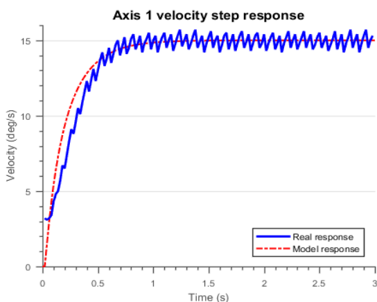
Fig. 7. Comparison of responses of the physical velocity control system and its model
