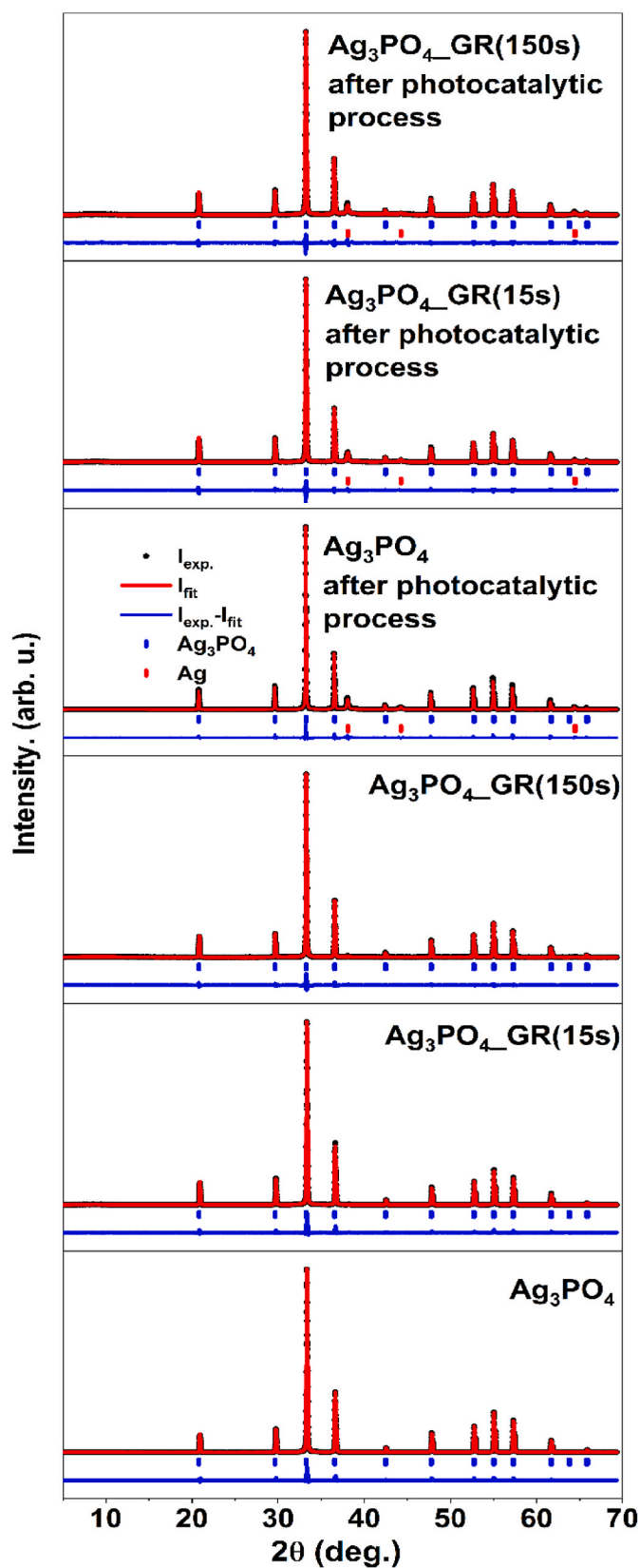
Fig. 7. Power X-ray diffraction patterns for \text{Ag}_3\text{PO}_4 , \text{Ag}_3\text{PO}_4 -GR(15s), \text{Ag}_3\text{PO}_4 -GR(150s), before and after the photocatalytic process of phenol degradation.
