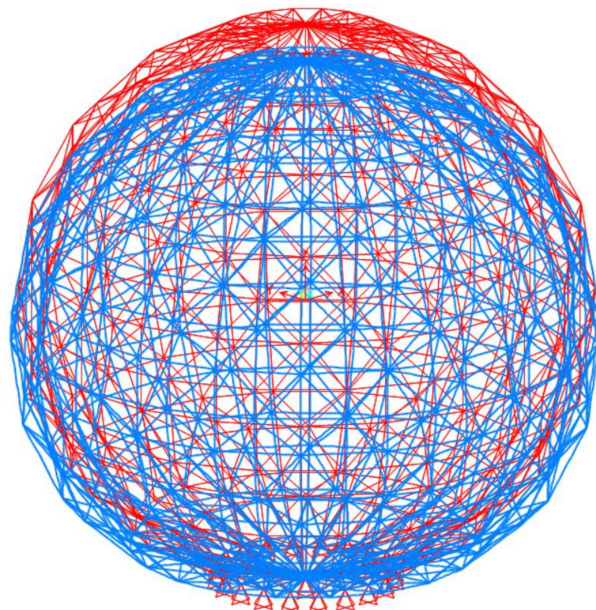
Fig. 3. Deformed shape of the spherical model after loading
