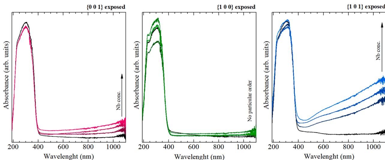
Fig. 5. DR/UV-vis absorption analysis for the obtained \text{TiO}_2 photocatalysts doped with Nb and exposed with different crystal facets.
