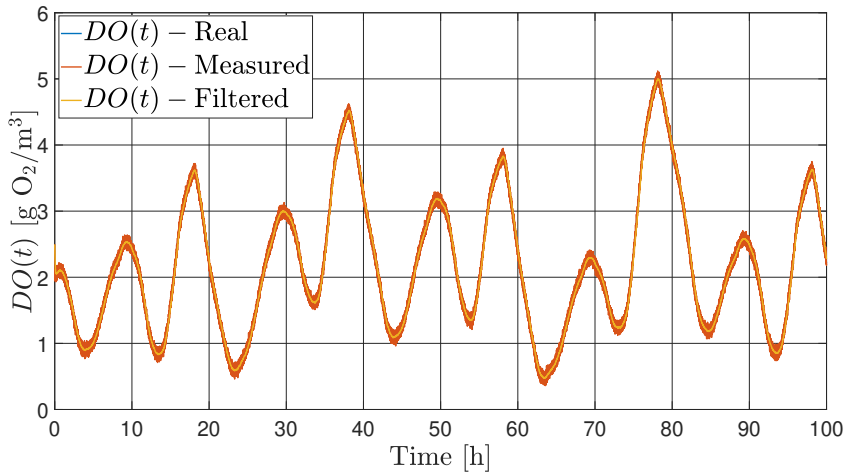
Figure 7: Trajectories of the dissolved oxygen concentration DO(t) .
