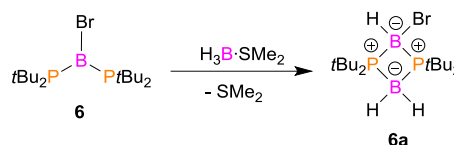
Scheme 4. The reaction of 6 with H_3B-SMe_2 .
