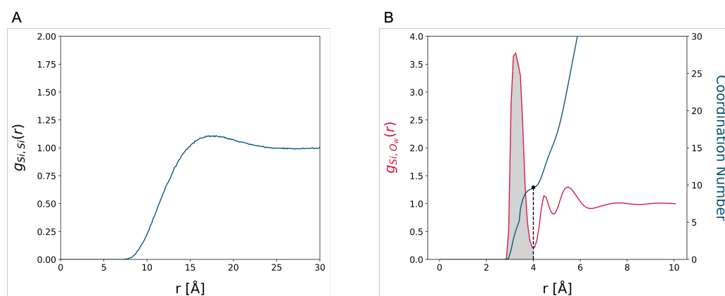
Figure 1. (A) Radial distribution function ( g(r) ) between silicon atoms of the water–silica system, depicting a broad, homogeneous distribution of \text{Si(OH)}_4 molecules. (B) Radial distribution function of the oxygen atoms of water about the silicon atoms of \text{Si(OH)}_4 (red line), displaying a peak about 3.5 Å. The blue line describes the cumulative distribution of the g(r) , with the shaded area under the peak quantifying the coordination number of \text{Si(OH)}_4 —that is, about 10 water molecules per molecule of orthosilicic acid.
