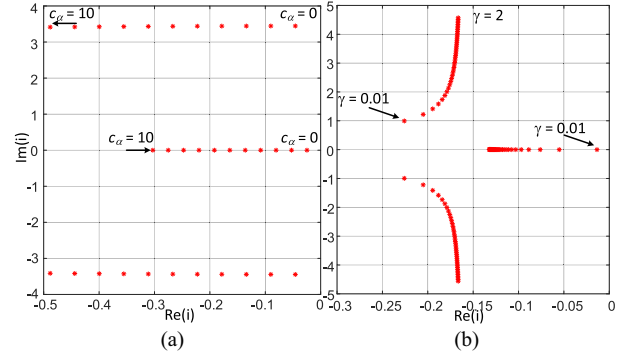
Fig. 5. Spectrum of matrix \mathbf{A} of the linearized observer system for c_\lambda = 0.05 , k_c = 0.5 , T_L = 1 , \omega_r = 1.0 p.u., c_\theta = 1 and for: (a) c_\alpha is changing from 0 to 10 p.u. and (b) \gamma is changing from 0.01 to 2.0 p.u. and c_\alpha = 3.0 p.u.
