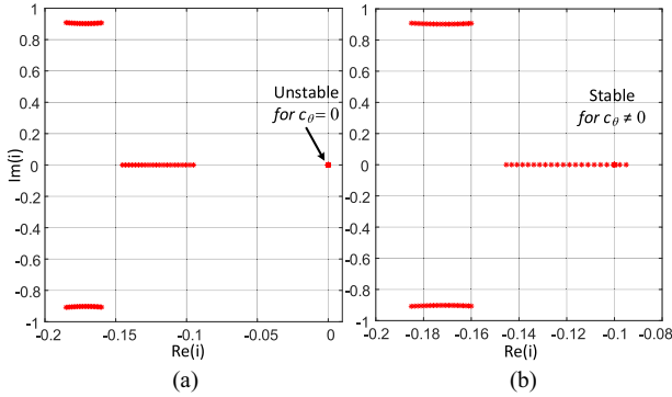
Fig. 3. Spectrum of matrix \mathbf{A} of the linearized observer system for c_\alpha = 3.0 , c_\lambda = 0.05 , k_c = 0.5 , T_L = 1 , \omega_r = 0 p.u. and (a) c_\theta = 0 , (b) c_\theta = 0.1 p.u.
