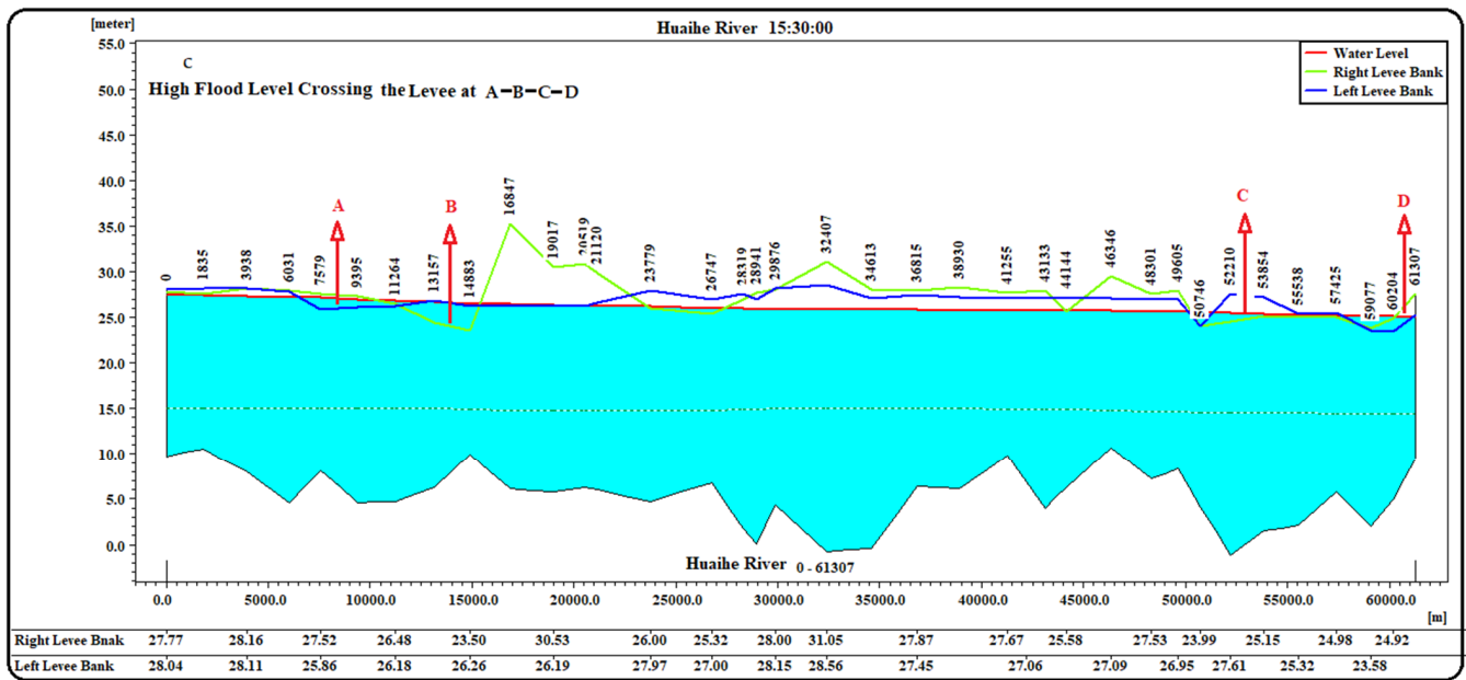
Figure 3. Profile view of simulated water level: indicating normal flow in figure (a), maximum flow line indicates high flood level in figure (b) and figure (c) shows dams breaking at A, B, C, and D points left and right levee.
