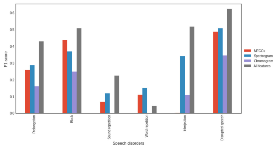
Figure 7. Values of the F1 measure for the baseline model on test set after training on specific features.
